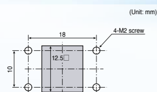
Installation dimensions(Unit:mm)
