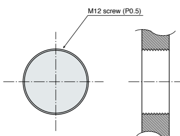
Installation dimensions(Unit:mm)
