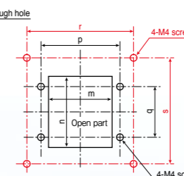
Black: Dimensions of thin element installation hole Red: Dimensions of rainproof cover installation hole
